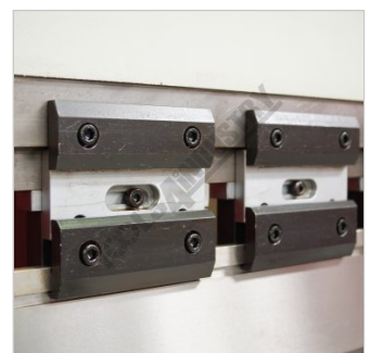
Intermediate Clamps
