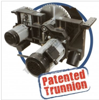
Trunnion
