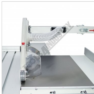
Tilting Blade Guard Front View
