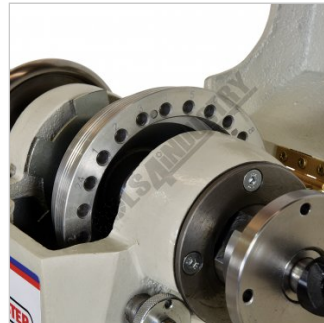
24 Position Indexing
