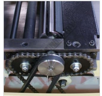
Chain Drive Feed Rollers
