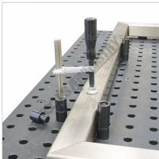
Optional SC 60 Clamp Shown Screwed into Threaded Adaptor View 2
