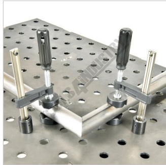
Round Tube Setup with Clamps and V Pads
