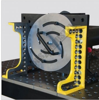
Being Used to Hold the Universal Flange Clamping Plate
