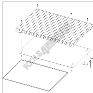
Assembly Drawing
