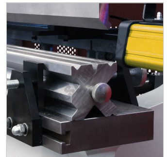
Top-Bottom Tooling
