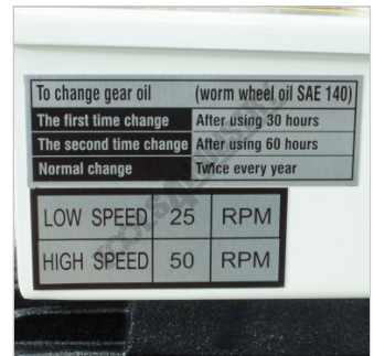
Blade Speeds
