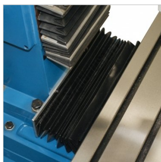
Concertina Slideway Covers
