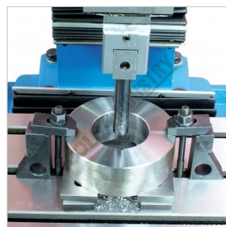
Shown Slotting Front View
