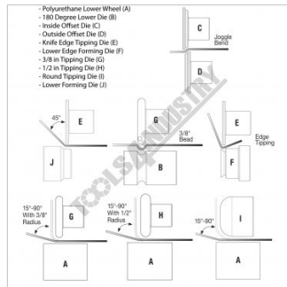
Examples of Metal Contours with Die Combinations
