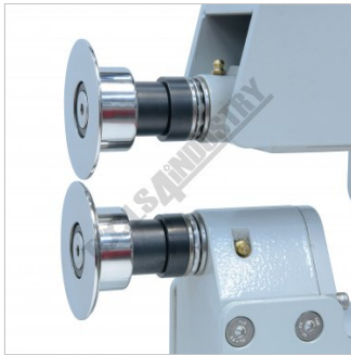
Inside Offset Die with Knife Edge Tipping Die
