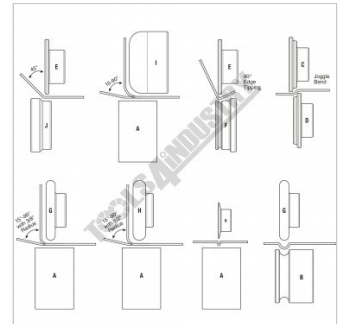
Examples of Metal Contours with Die Combinations
