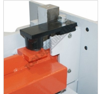
Material Clamp
