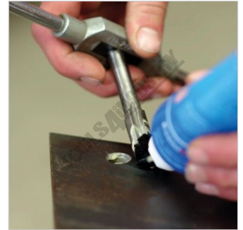
Tapping Action Close Up
