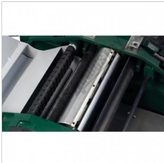
Cutter Block
