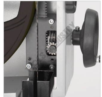
Toolpost Support
