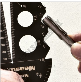
Thread Checker
