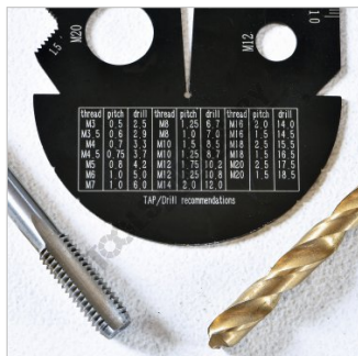
Tap-Drill Chart
