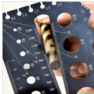
Drill Diameter
