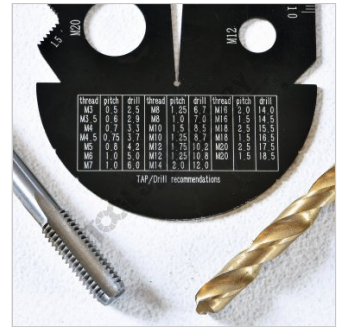
Tap-Drill Chart
