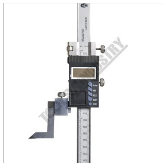
Display & Controls
