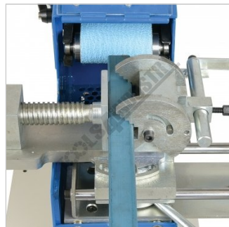
Square Vice Jaws Holding Round Material at 90 Degrees
