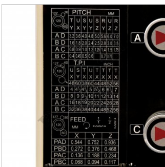
Thread-Feed Chart
