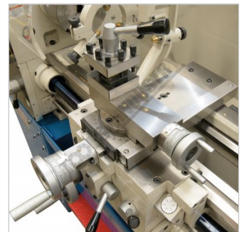
Compound Slide
