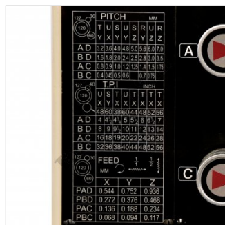
Thread-Feed Chart
