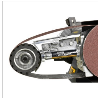
Belt Adjustment
