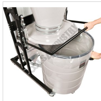
Quick Release Bucket
