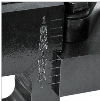
Adjustable Tool Height Setting
