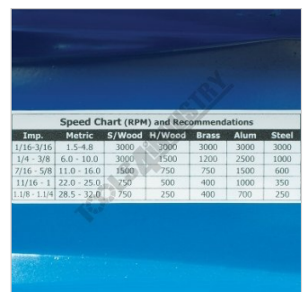
Recommended Speed for Drill Size and Material
