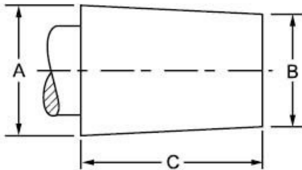
JACOBS TAPER SPECIFICATIONS
