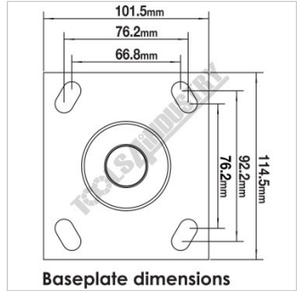
Baseplate Dimensions
