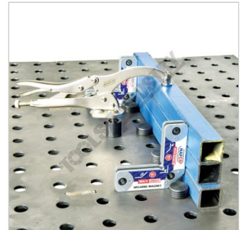
Square Tube Setup with Clamp on Optional Riser
