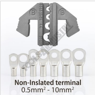
Non Insulated Terminal Jaw 0.5mm 2 - 10mm 2
