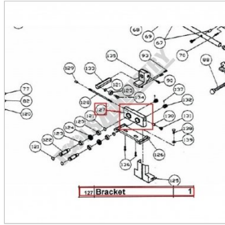
Parts Diagram
