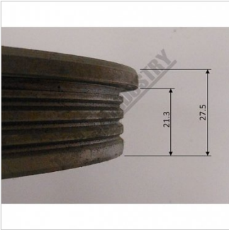
BF109 WHEEL OD 364 BORE 52.2
