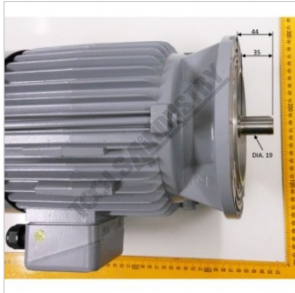
5BM0116 MOTOR 415V 7A 2.3
