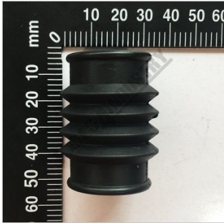
Rubber Cover
