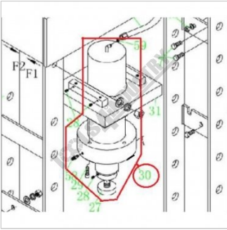
4PR0030 CYLINDER ASSY 30
