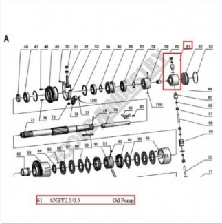
4LS1061 OIL PUMP SNBY2.5 0
