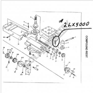
2LX5000 Assembly
